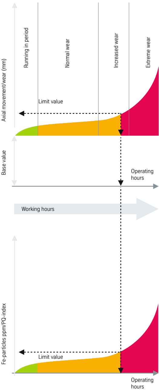
Figure 46: Wear curves
