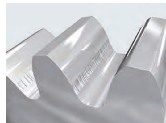
Figure 22: Scuffing
