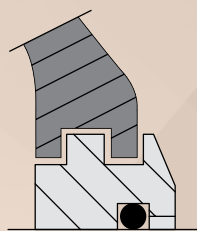
LABYRINTH (LO)
